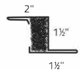
17. Snap-Z150 Vented Closure
