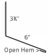
6. Endwall Flashing
