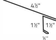
15. Residential Eave
