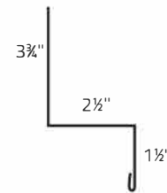
5. Sidewall Flashing
