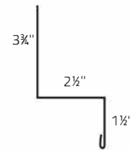
5. Sidewall Flashing
