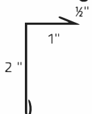
13. Counter Flashing
