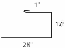
7. Starter J
