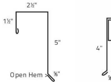
3. Gable Flashing
