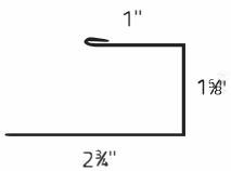
7. Starter J
